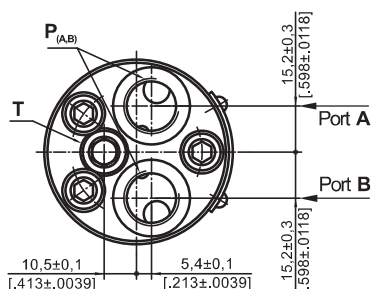
Rear Ports
