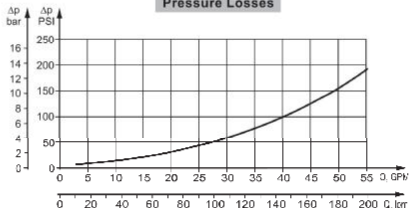
Pressure Losses
